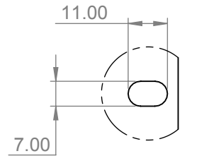
DETAIL A SCALE 2 : 3
